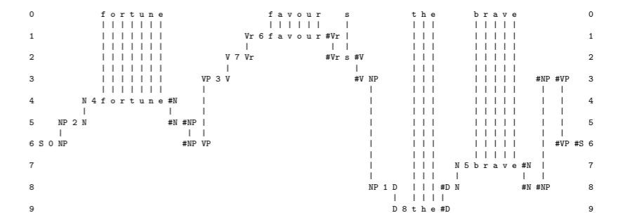
Figure 3: An SP-multiple-alignment that represents a parsing of the sentence “Fortune favours the brave”.
